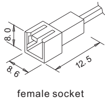
female socket
